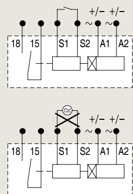
Circuit diagram
