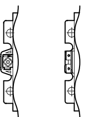
Screw clamp
